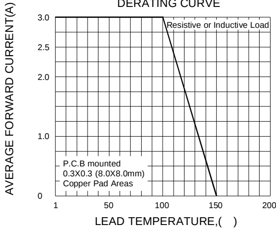
F1G.1-FORWARD CURRENT DERATING CURVE
