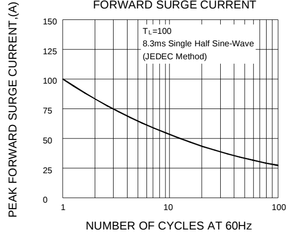
F1G.2-MAXIMUM NON-REPETITIVE PEAK FORWARD SURGE CURRENT
